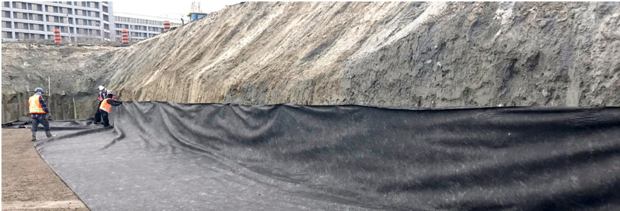
Excavation and geotextile at nearly 5m deep
