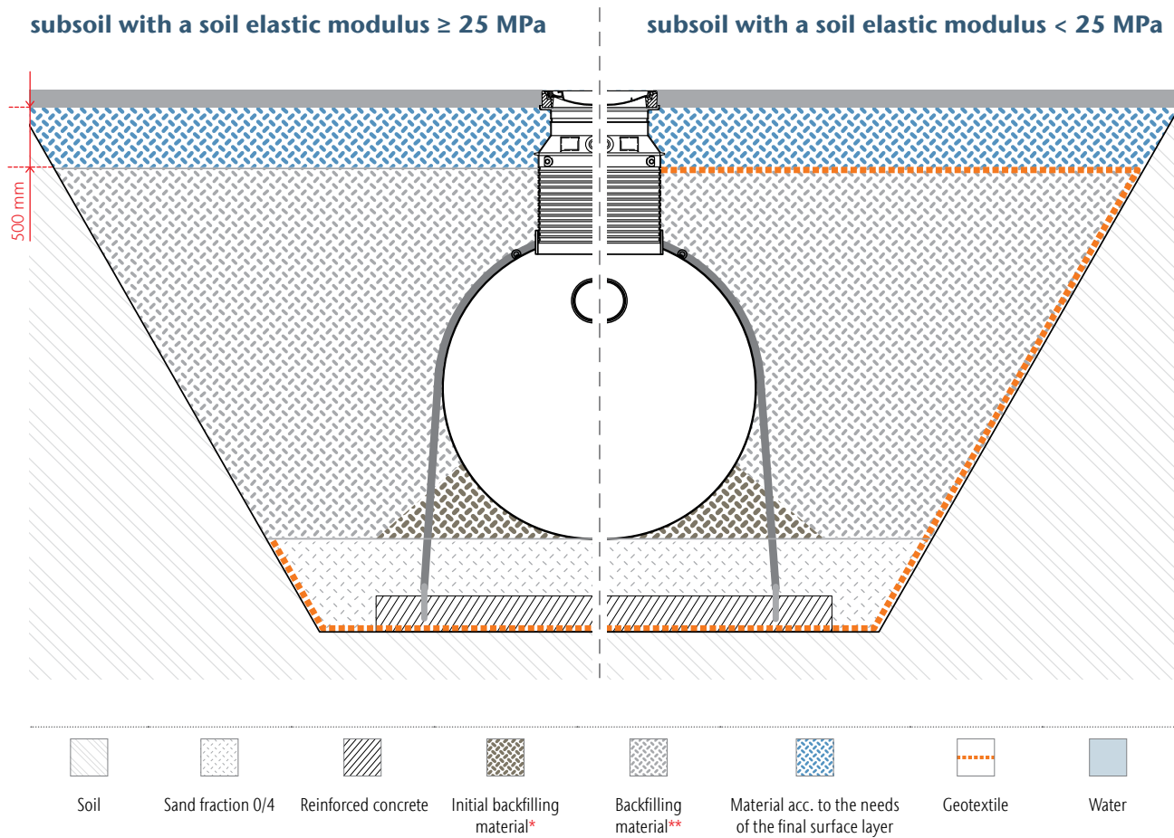
Figure 10.6 Backfilling and geotextile
