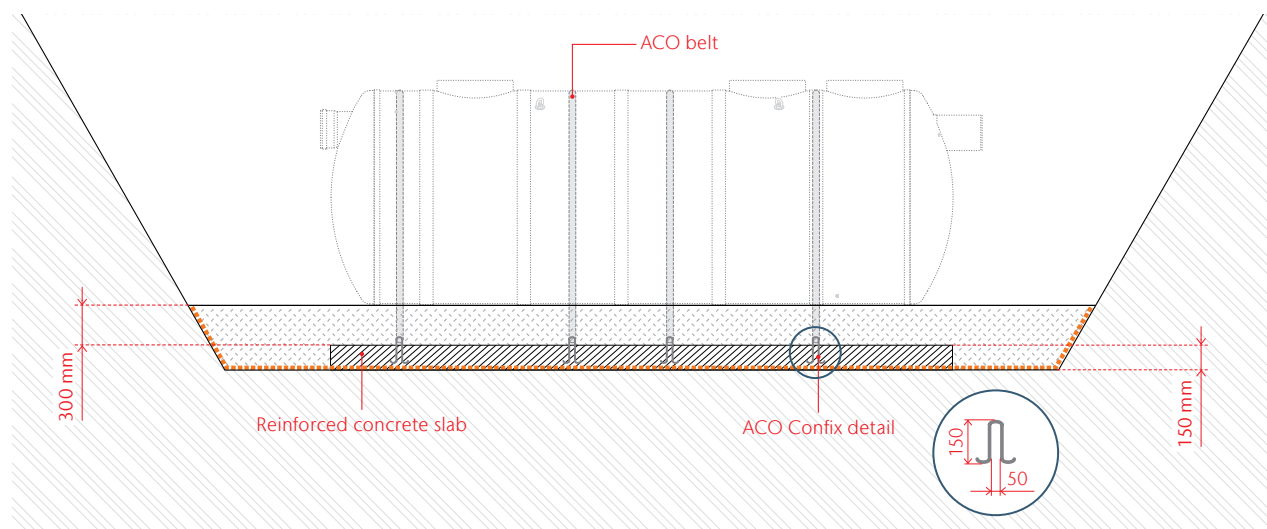
Figure 8.5 Dimensions of the reinforced concrete slab
