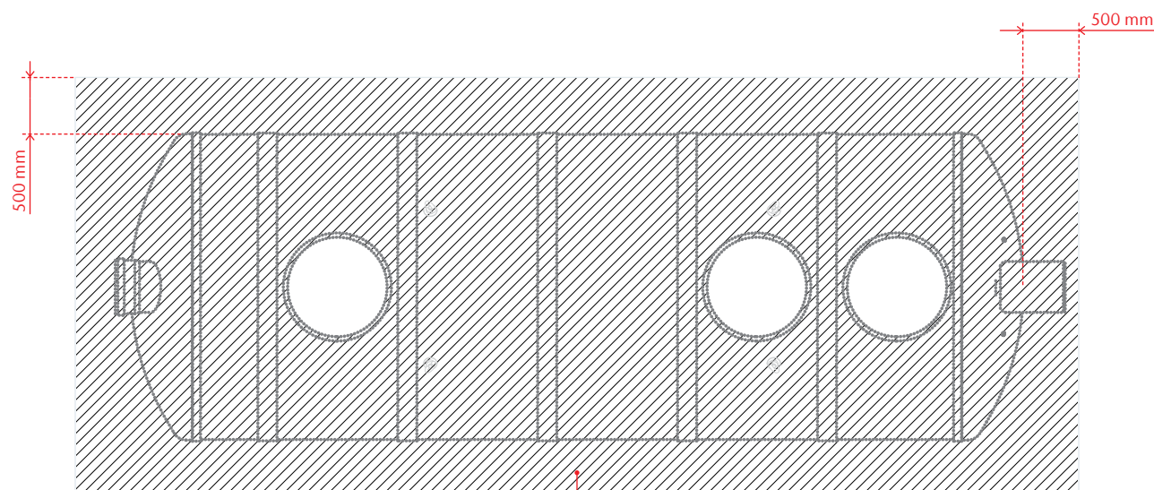
Figure 10.11 Reinforced concrete load distribution slab
