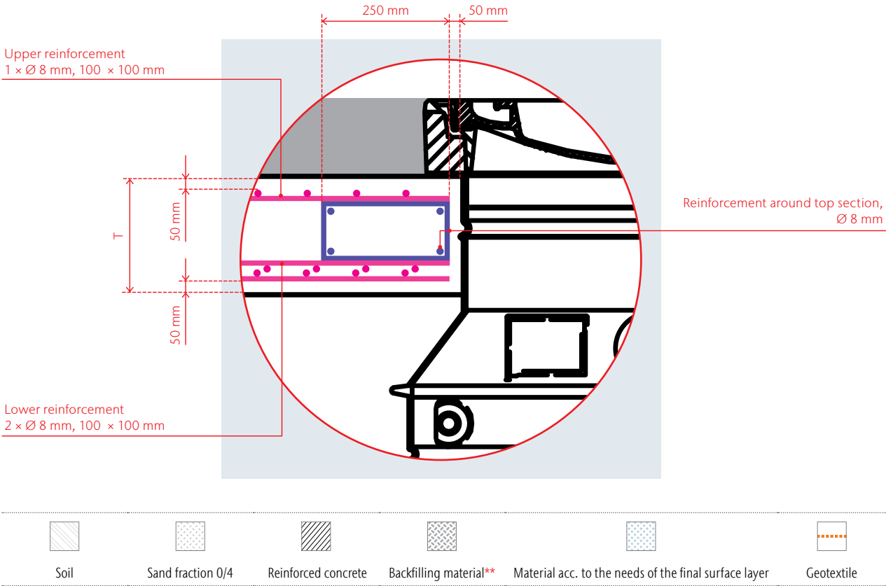
Figure 10.13 Reinforcement in the concrete slab
