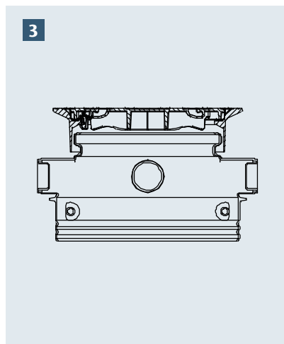
3 DN 600 load class A with short floating cover
