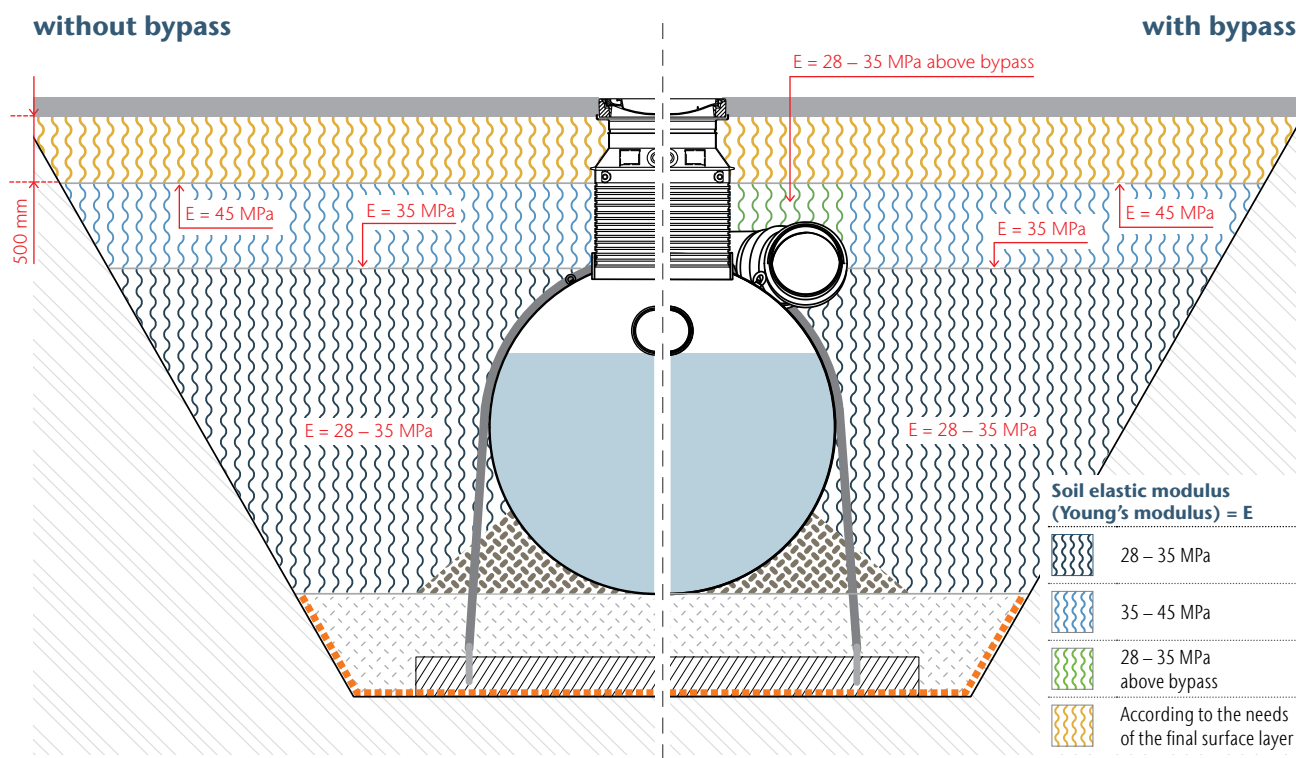
Figure 10.6 Backfilling and geotextile
