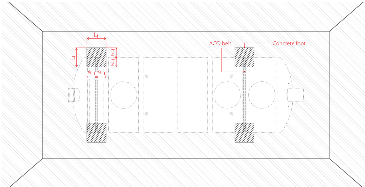
Figure 8.2 Dimensions of the concrete feet
