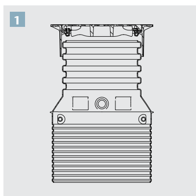
1 DN 600 load class A/B with floating cover
