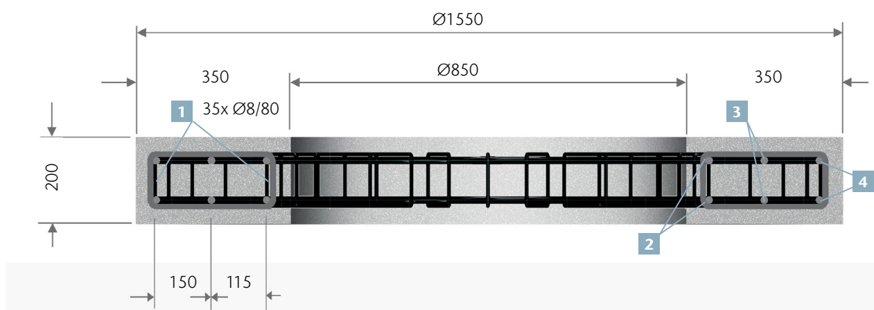
Figure 10.17 Cross section
