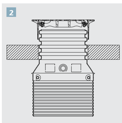
2 DN 600 load class D (with load distribution ring) with floating cover
