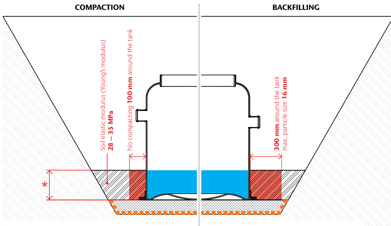
Figure 9.4 Backfilling with crushed stone or native soil
