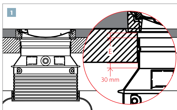
Figure 10.10 Concrete ring installation
