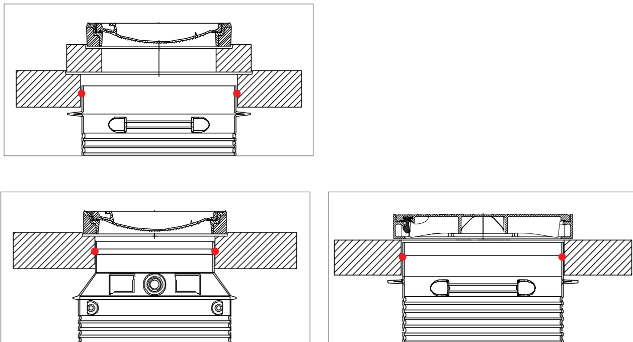
Figure 10.11 O-ring rubber installation
