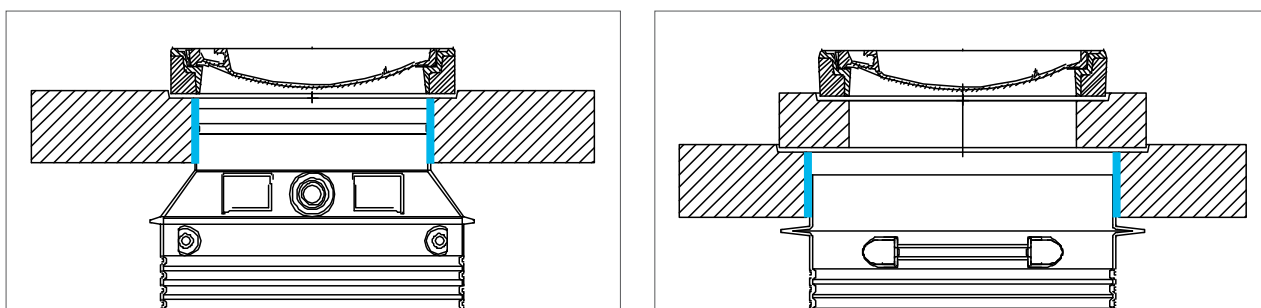
Figure 10.12 Expansion strip placement
