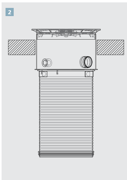
2 DN 800 (manhole cover DN 800) load class D (with load distribution ring) with floating cover
