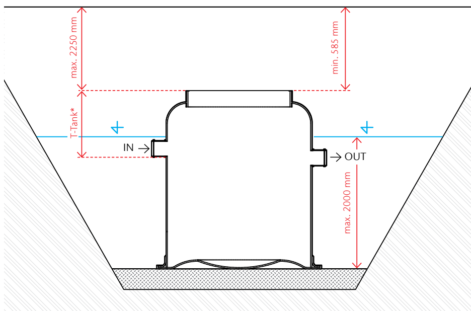
Figure 4.1 General installation information
