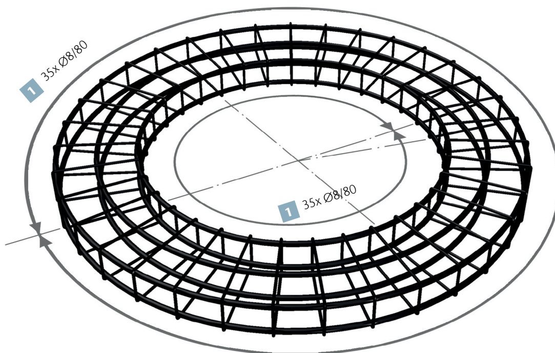
Figure 10.16 Reinforcement plan for the load distribution reinforcement concrete ring DN 800
