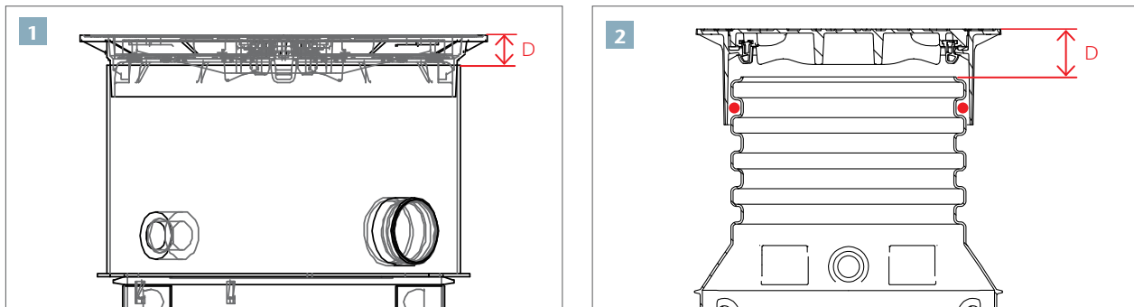
1 Top section DN 800 with floating cover Dimension D = 80 mm
